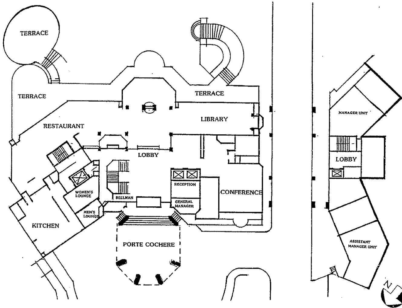
LOBBY LEVEL
