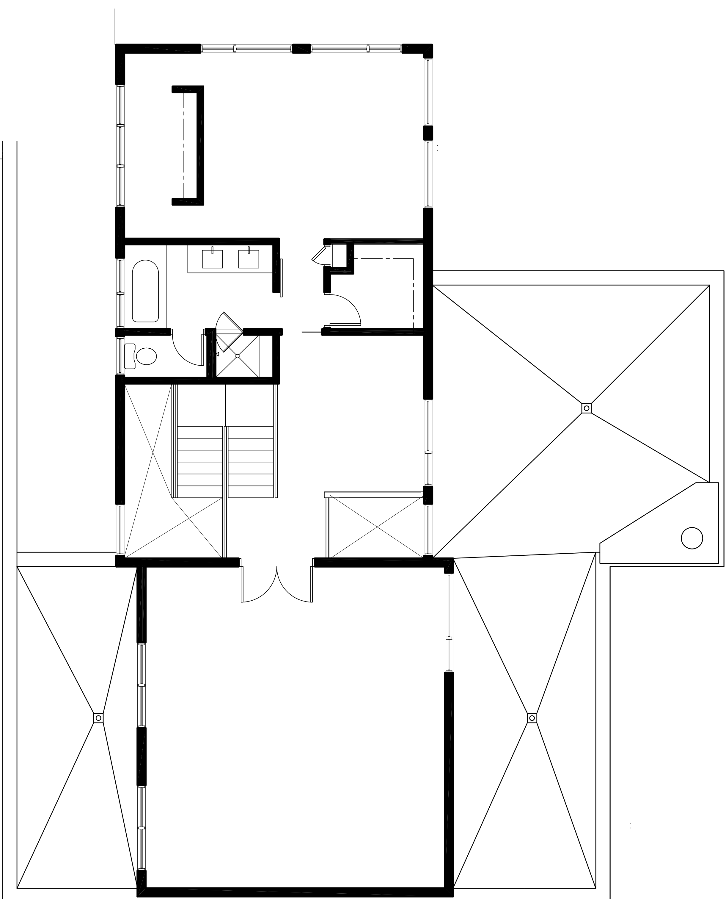
UPPER LEVEL PLAN 1/4" = 1'-0"
