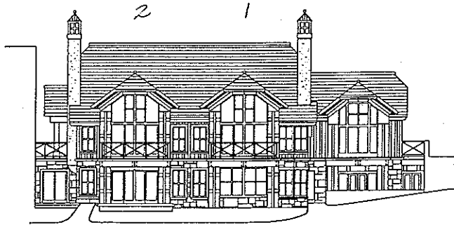
WEST ELEVATION - VILLAS B - A
